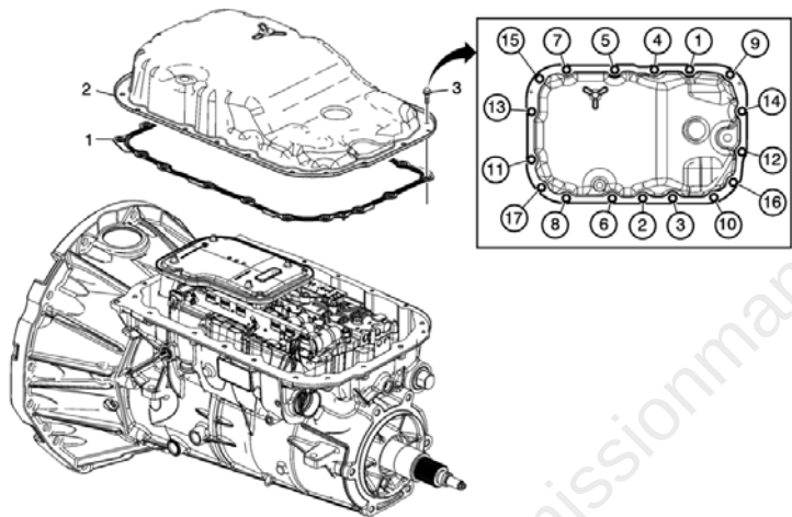
Transmission Fluid Pan Installation
